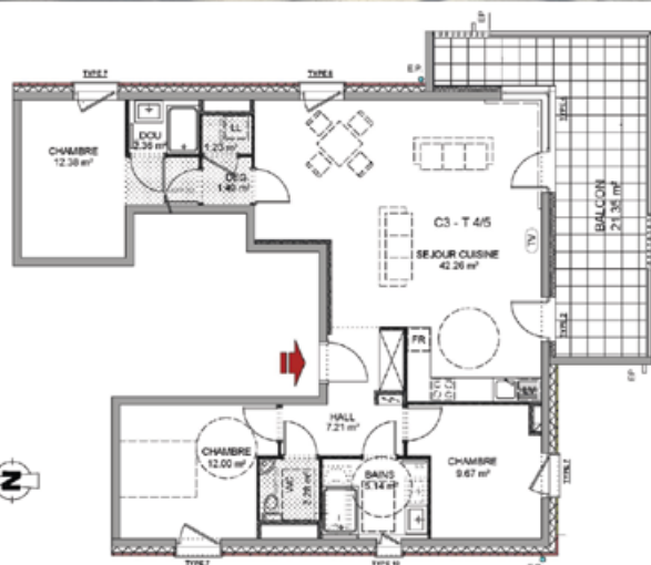
LOT C3 - 4/5 pièces
